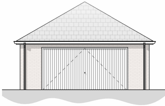
North Elevation 1 : 100
